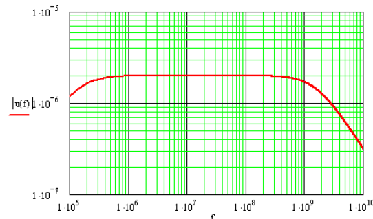
Figure 3 : Response of the full system (relation output voltage / E field)
