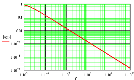
Figure 2 : Response of the integrator alone (output voltage / input voltage)
