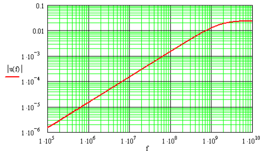
Figure 1 : Response of the sensor alone (relation output voltage / E field)
